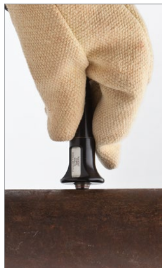
D790-SM transducer on a high-temperature pipe
