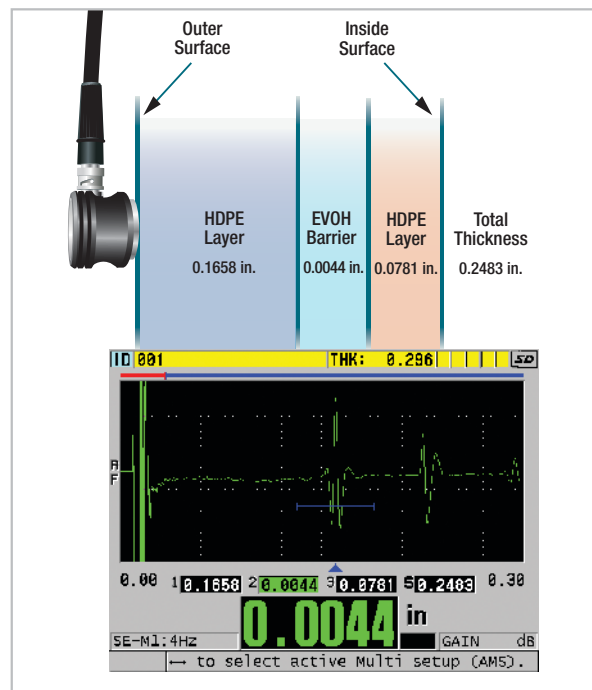
The 38DL PLUS thickness gage can make accurate measurements of up to four individual layers simultaneously.
